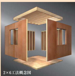
2×6工法概念図
